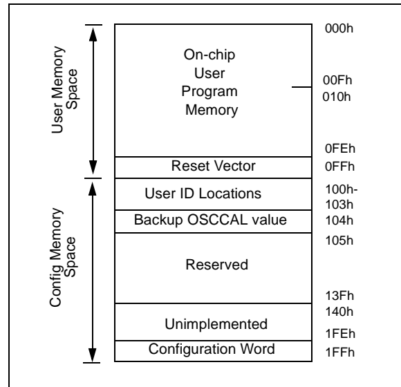
FIGURE 2-1: PIC10F200/204 PROGRAM MEMORY MAP
