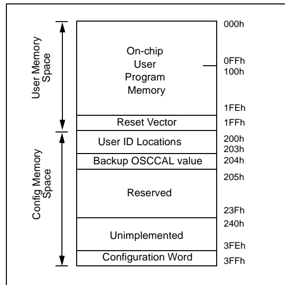
FIGURE 2-2: PIC10F202/206 PROGRAM MEMORY MAP
